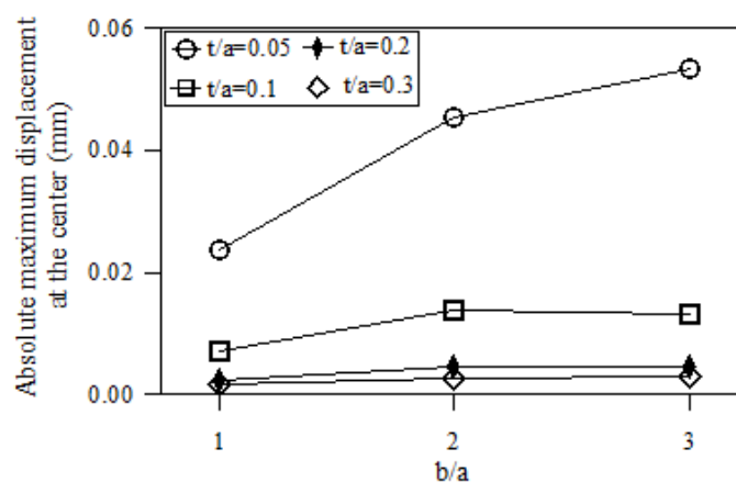
Fig. 6. Absolute maximum displacement of the thick clamped plates resting on Winkler foundation for different aspect ratios and thickness/span ratios.
