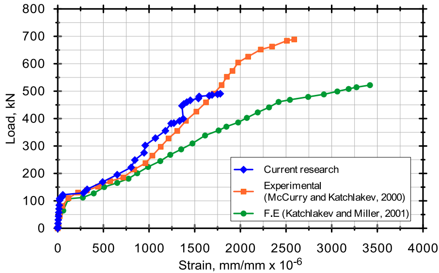
Figure 17: Load strain curve in the GFRP for the shear beam.
