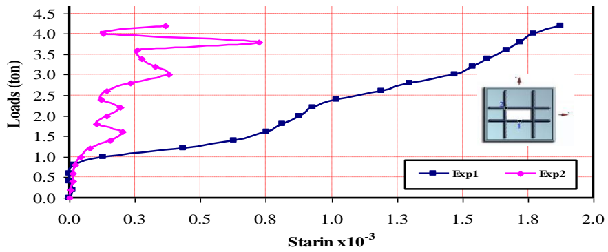
Figure 10-a Load-CFRP Strain Curves for S_tMC_eCO
