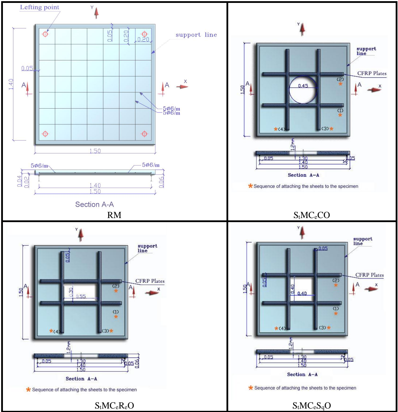
Figure 1-a Layout of rebar, CFRP arrangement and model geometry
