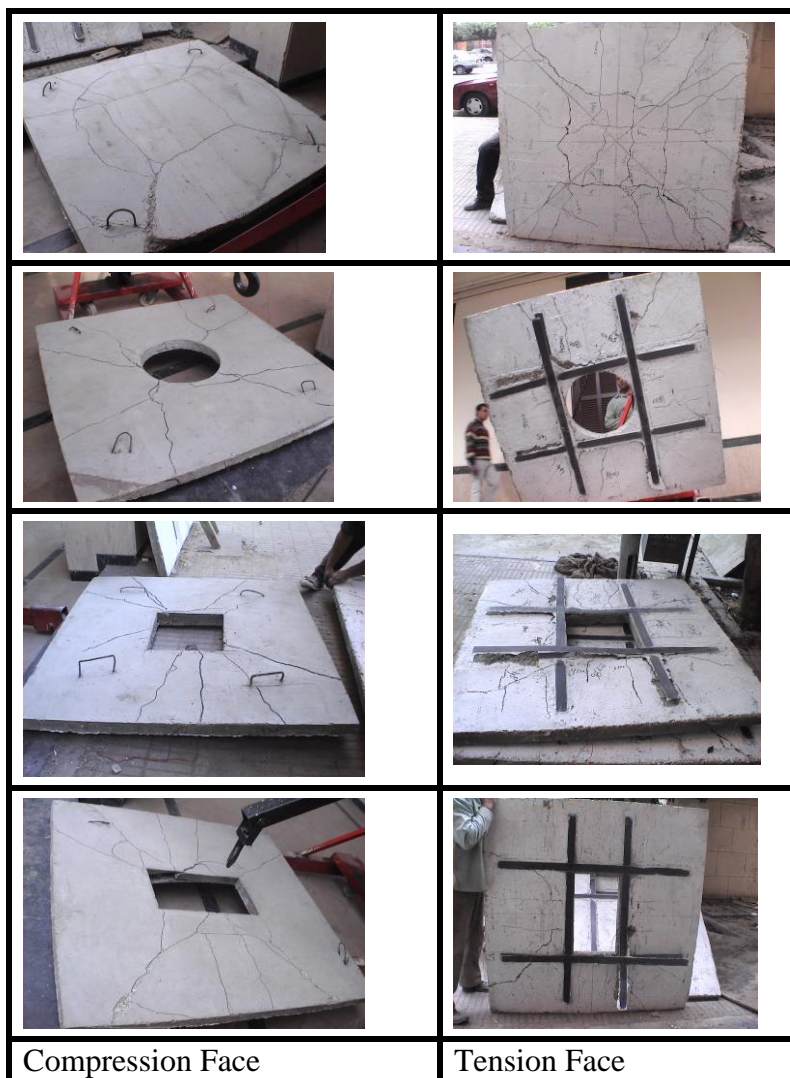
Figure 4- Crack Patterns
