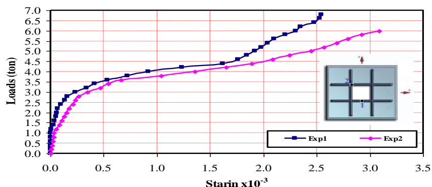
Figure 10-c Load-CFRP Strain Curves for S_tMC_eS_qO
