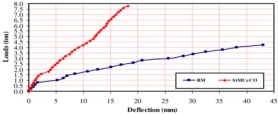
Figure 7-a Load-Deflection Curves for RM and S_tMC_eCO
