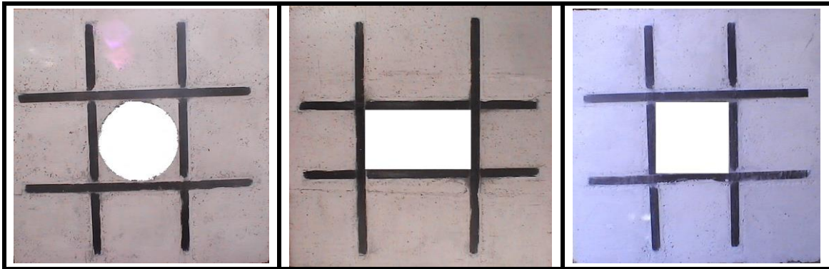
Figure 2- CFRP Laminates on tension face of models with opening
