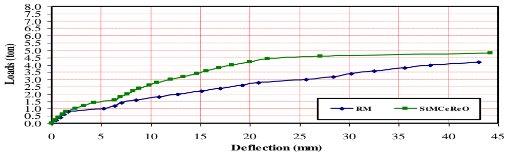
Figure 7-b Load-Deflection Curves for RM and S_tMC_eReO
