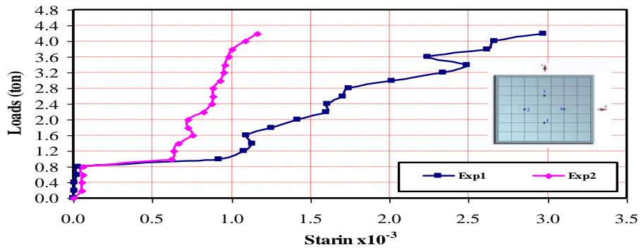
Figure 9-a Load-Steel Strain Curves for RM
