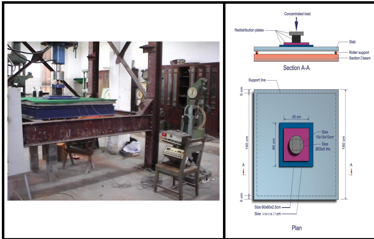
Figure 3 - Test Setup
