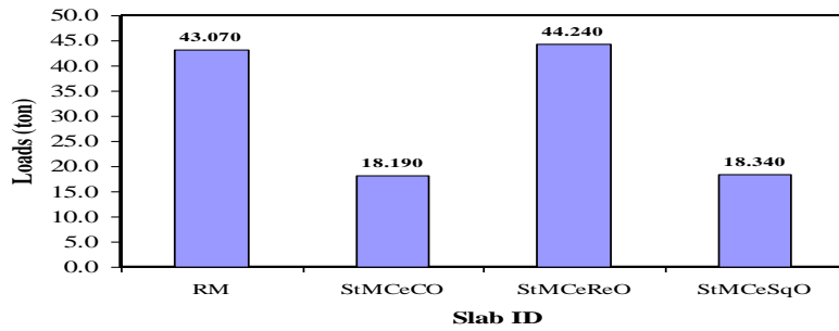
Figure 8-a Max. Deflection for RM and Other Models
