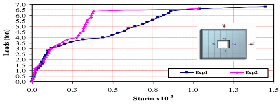
Figure 9-d Load-Steel Strain Curves for S_tMC_eS_qO
