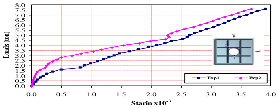
Figure 10-a Load-CFRP Strain Curves for S_tMC_eCO
