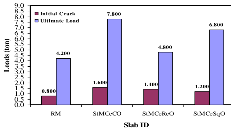
Figure 8-b Initial Crack Load and Ultimate Loads for RM and other Models
