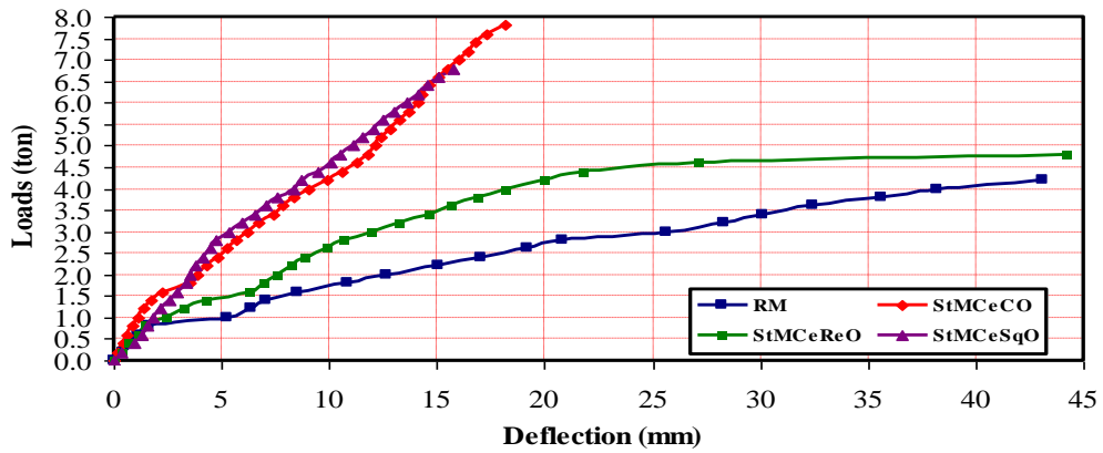
Figure 7-d Load-Deflection Curves for RM and other Models
