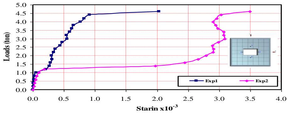
Figure 9-b Load-Steel Strain Curves for S t MC c CO
