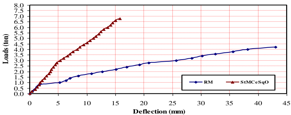
Figure 7-c Load-Deflection Curves for RM and S_tMC_eSqO
