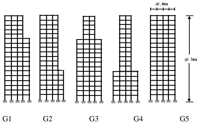
Figure 16: Elevation of different geometries of 18 storey test structures
