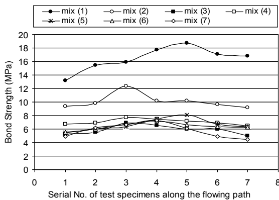
Fig. 6. Bond strength along the flow path (10 mm bar diameter specimens)
