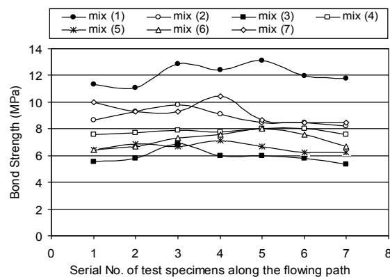
Fig. 7. Bond strength along the flow path (16 mm bar diameter specimens)
