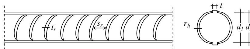
Fig. 2. Geometry of the steel bars
