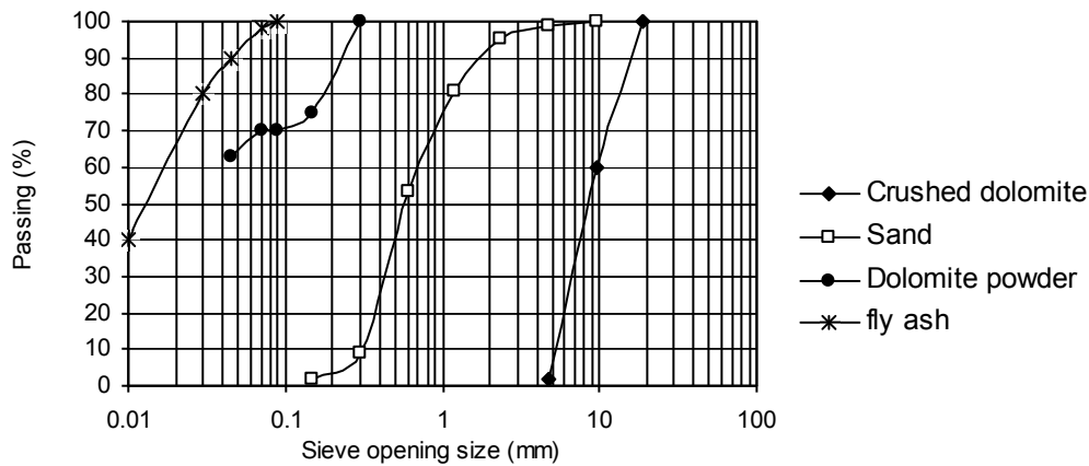
Fig. 1. Particle size distribution for concrete materials
