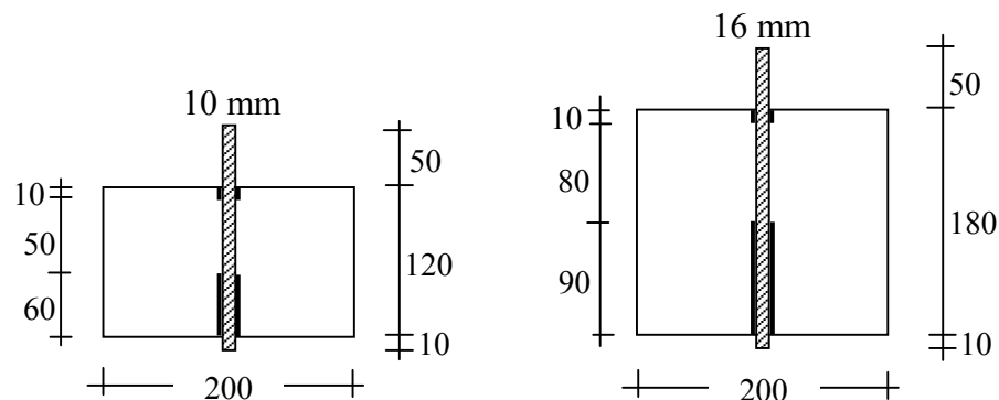
Fig. 3: Configuration of push-out bond test specimens
