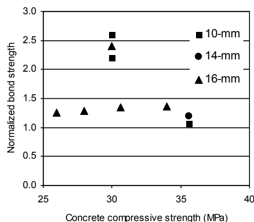
Fig. 5. Normalized bond strength and corresponding compressive strength
