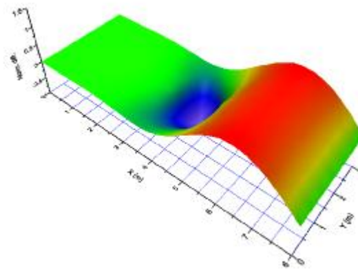
Figure 12: Isometric view of the smoothed surface of the mode 2 difference
