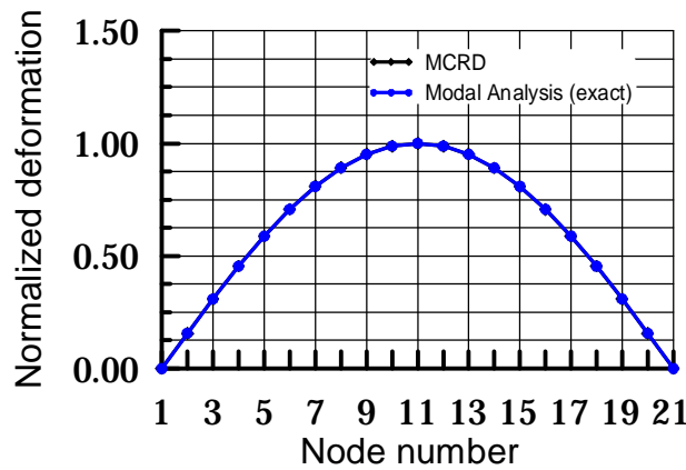
Figure 5: Mode 1 comparison (MCRD vs. Exact)
