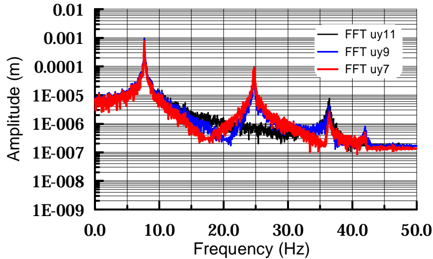
Figure 4: FFT of the response at points 11, 9, and 7 due to load application at point 5
