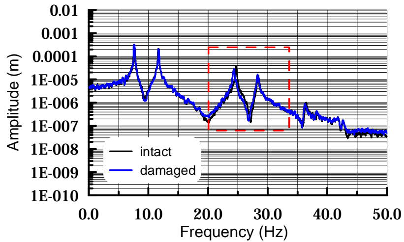
Figure 7: FFT at point 7 for intact and damaged beam
