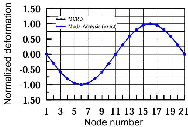
Figure 6: Mode 2 comparison (MCRD vs. Exact)
