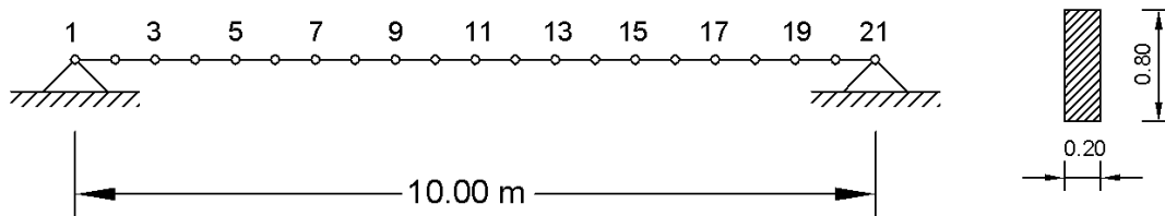
Figure 3: Single span beam dimensions
