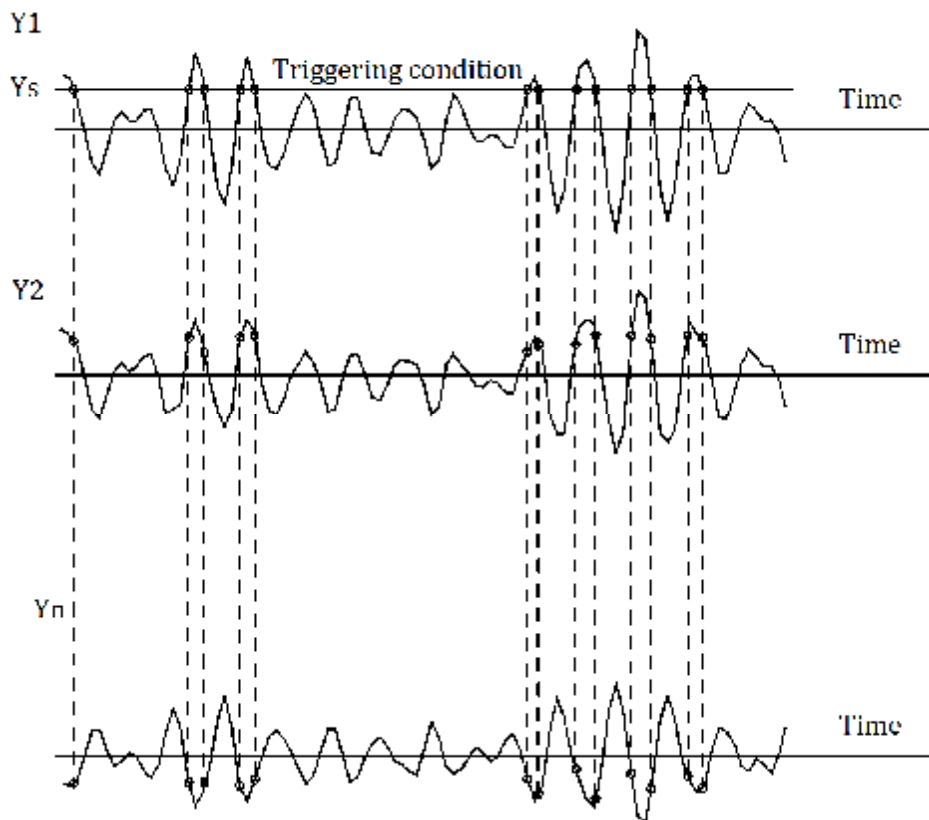
Figure 1: Multi-channel random decrement approach
